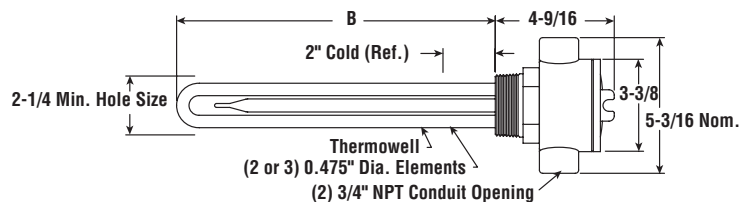
E4TP — Dimensions (Inches)
