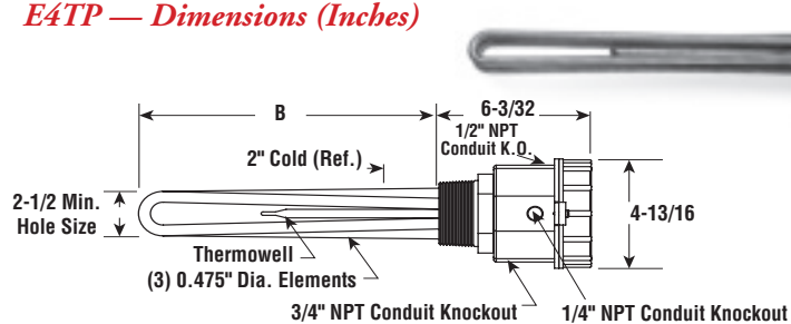
E4TP — Dimensions (Inches)
